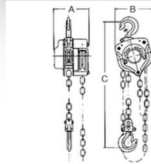
Chain Hoists Diagram
