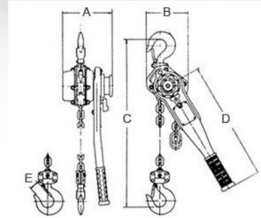
Lever Hoists Diagram
